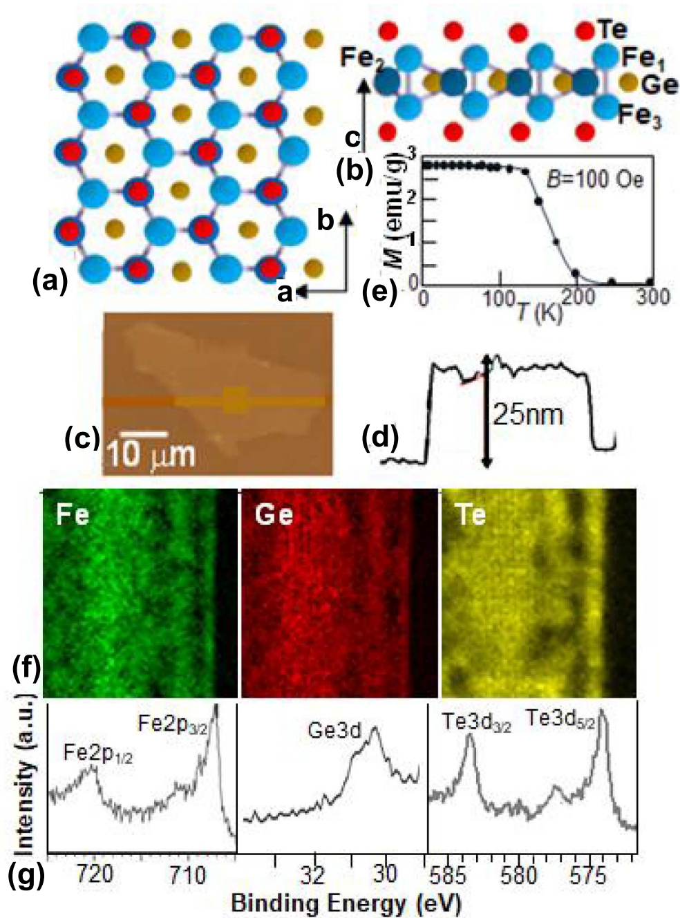
Figure 1. Schematic views of the atomic structure of FGT for (a) the x - y plane and (b) the z direction. Examples of (c) optical and (d) cross-sectional atomic force microscope images for an FGT flake. (e) An example of magnetization curve on temperature change. (f), (g) Examples of EELS mapping for each element (f) and XPS measurement (g).
