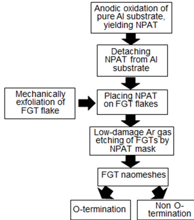
Figure 2. Sample preparation flow chart.
