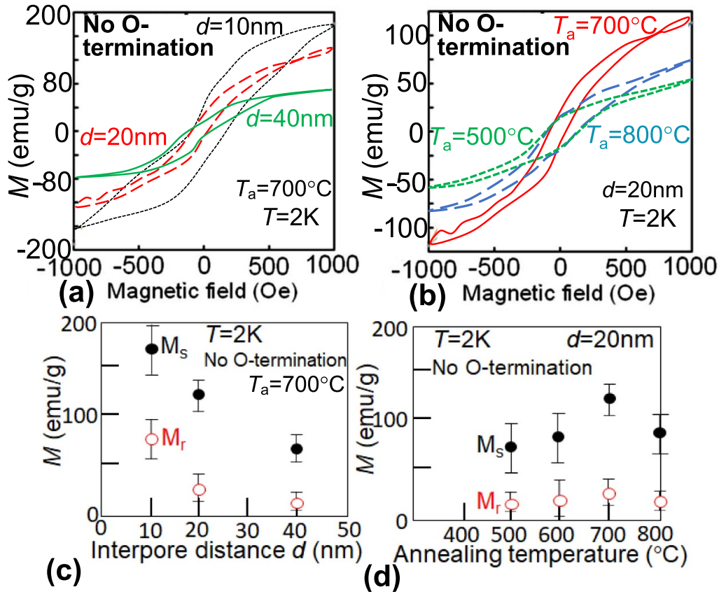
Figure 5. Magnetization curves for three different (a) mean inter pore distance ( d ) and (b) annealing temperature ( T_a ) for non-O-terminated FGT nanomeshes. For (a), black- and red-dotted, and green-solid curves correspond to d \sim 10, 20 and 40 nm, respectively. For (b), blue- and green-dotted, and red-solid curves correspond to T_a \sim 800, 500 , and 700 °C, respectively. Dependence of M_s and M_r values on (c) d obtained from (a) and (d) T_a obtained from (b) for non-O-terminated FGT nanomeshes.
