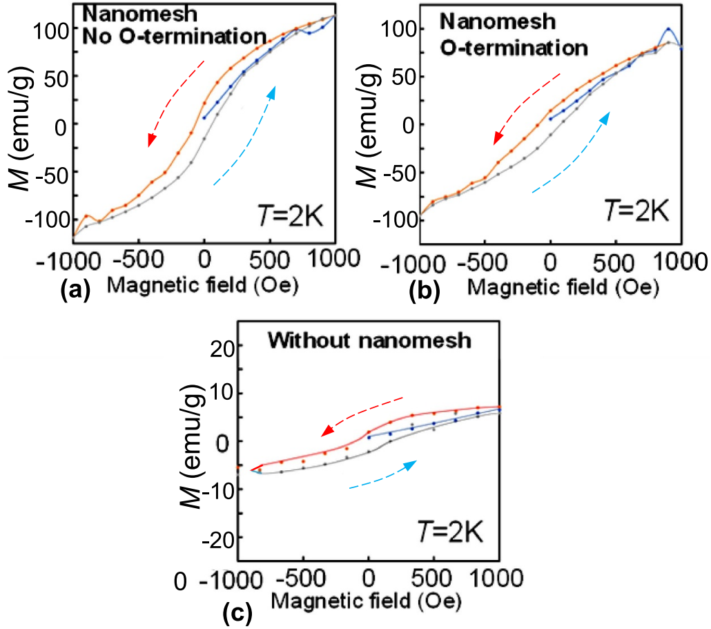
Figure 4. Examples of the magnetization curves for (a) non-O-terminated FGT-nanomesh(NM), (b) O-terminated FGT-NM, and (c) exfoliated pristine thin bulk flake. For (a) and (b), interpore distance ( d ) is \sim 20 nm and annealing temperature ( T_a ) is 700^\circ\text{C} . Magnetic field was applied along the c -axis (figure 1(b)) ( i.e. longitudinal direction of the nanopores).
