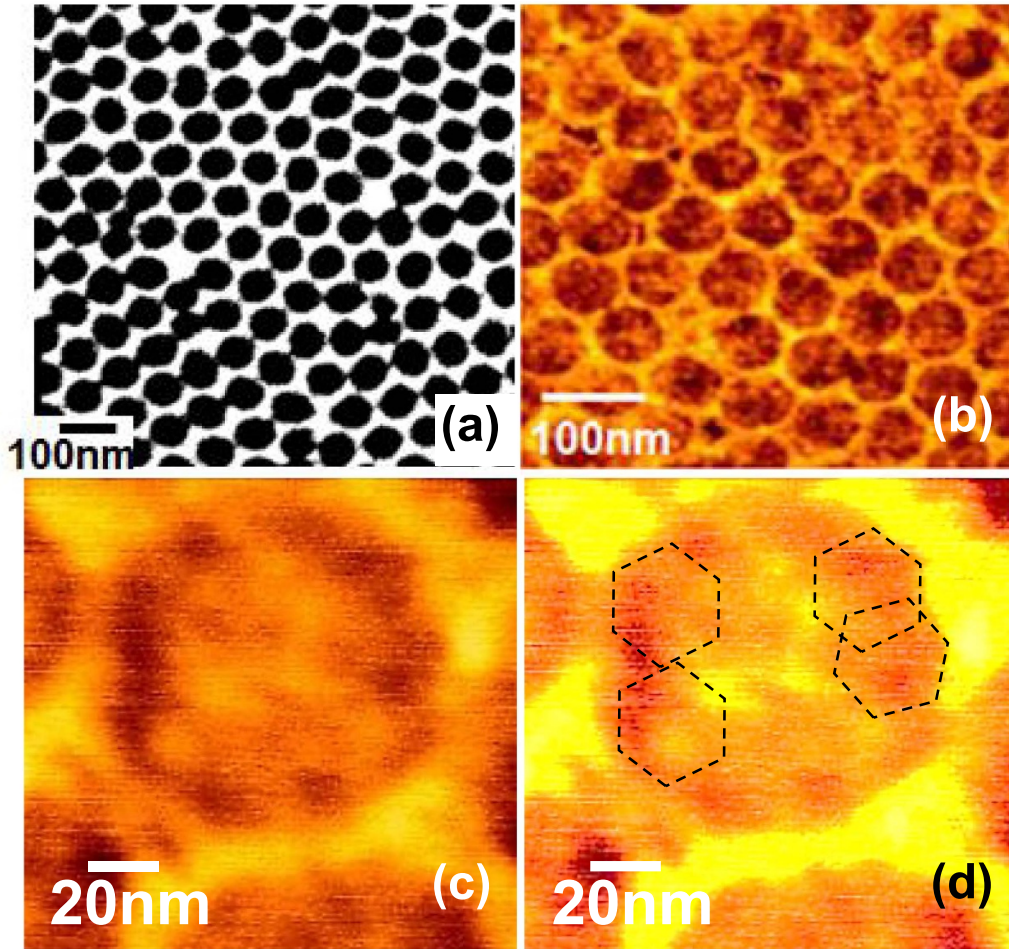
Figure 3. Examples of (a) SEM image of an NPAT mask and (b) a planer atomic force microscope image of an FGT nanomesh fabricated using (a). (c) Higher-resolution image of one pore in (b) and (d) its high-contrast image. Dotted hexagons in (d) are just to guide to eyes to confirm the angle \sim 120^\circ of the pore edges.
